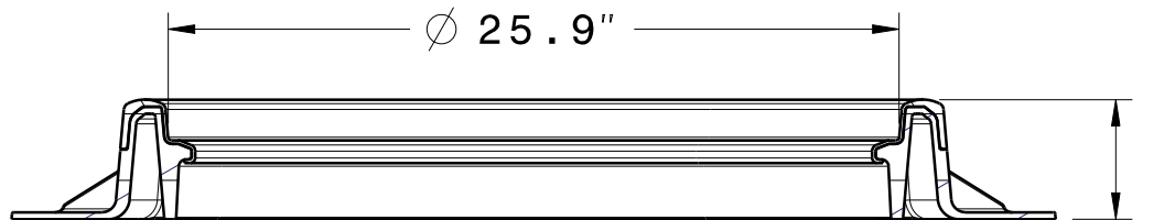
Section view A-A
